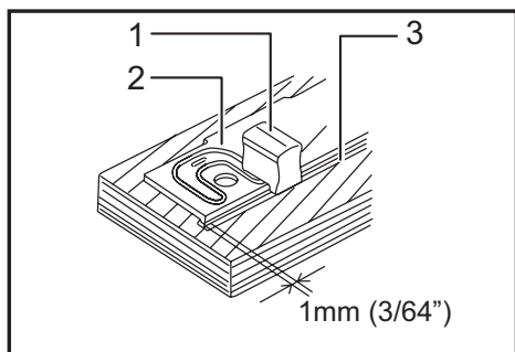
► 1. Magnetic holder 2. Set plate 3. Blade
