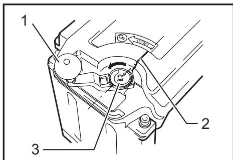
► 1. Crank handle 2. Groove 3. Depth adjusting gauge
