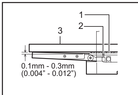
► 1. Post card 2. Adjusting screw 3. Ruler
